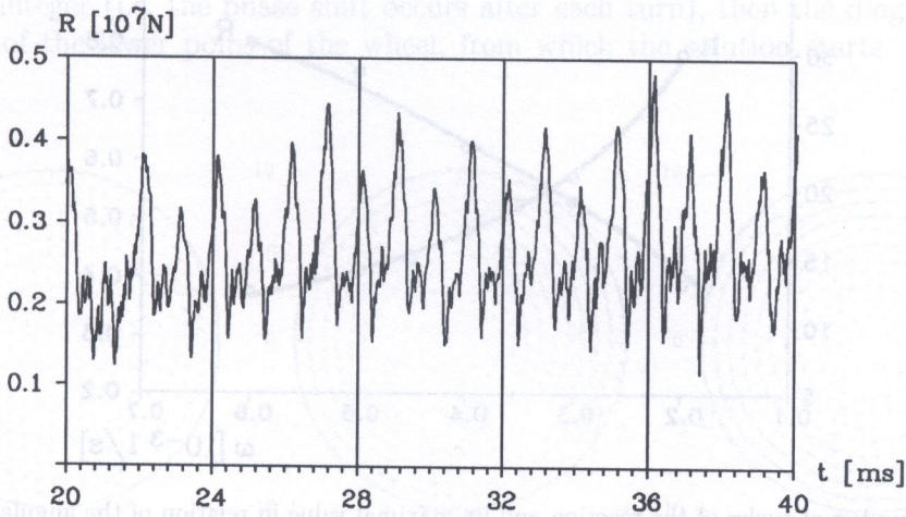
Fig. 13. The part of the diagram of the contact force in time
