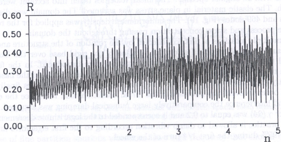
Fig. 12. Contact force in successive turns in the case of \omega = 0.3 \cdot 10^{-3} rad/s
