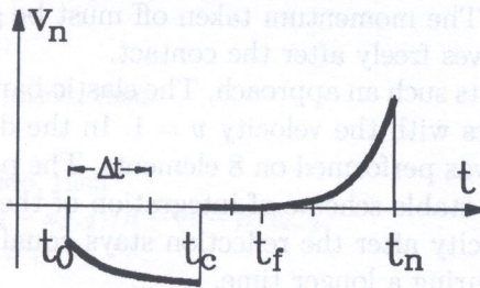
Fig. 6. Relative normal velocity in the time interval [t_0, t_1]
