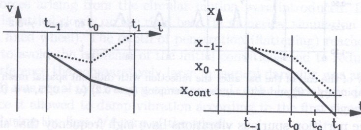
Fig. 7. Reduction of the velocity near the contact: continuous line – free motion, dashed line – motion with constraints
